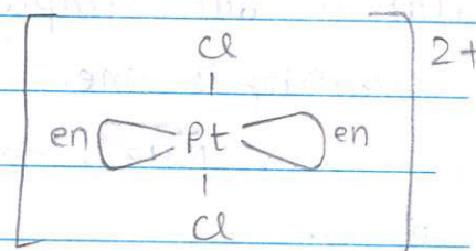
Trans-isomer
