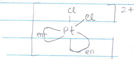
Cis-isomer
